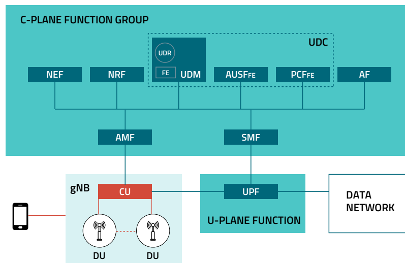
Figure 5: 5G CN is Agile and Cost-Effective to Operate
