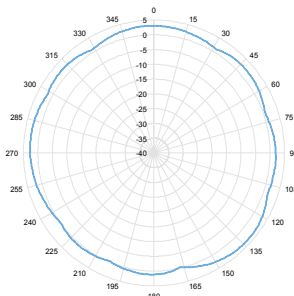
2.4 GHz Elevation
