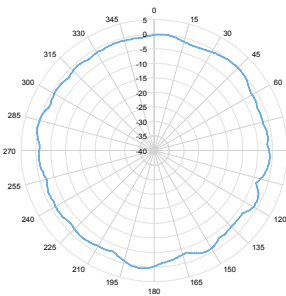
2.4 GHz Azimuth
