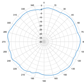
5 GHz Azimuth
