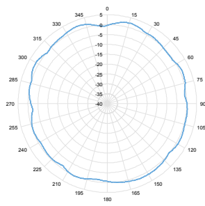
5 GHz Elevation
