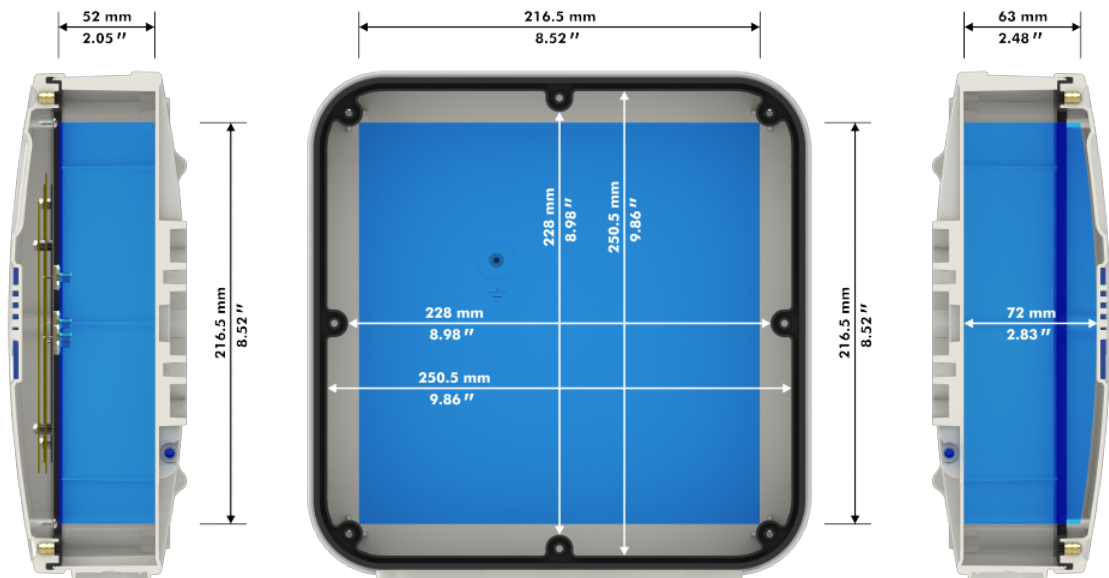
Inner dimensions WiBOX Medium
