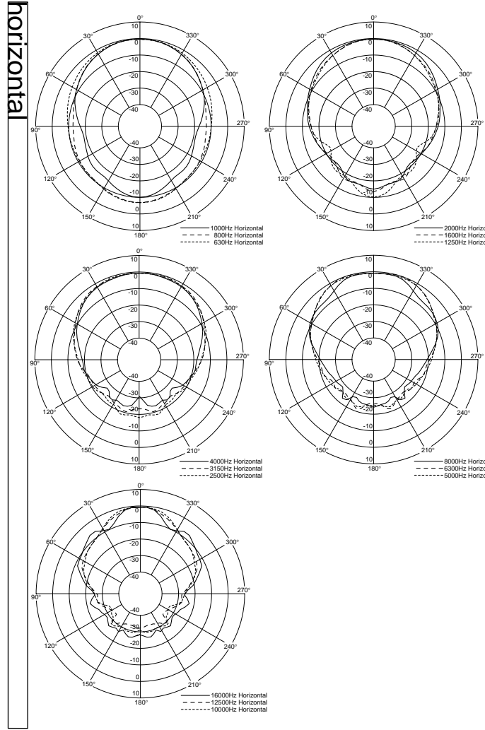
Polar Response
