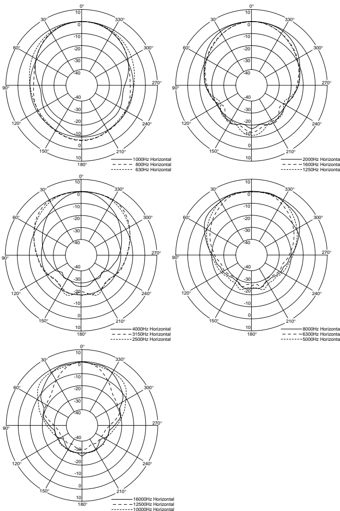
Polar Response
