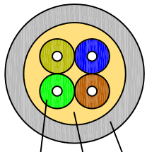
CABLE CONSTRUCTION
