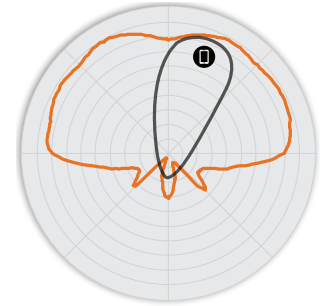
Figure 5. E510 5GHz Elevation Antenna Patterns
