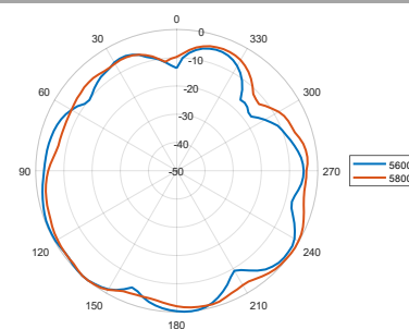
Elevation (Side View): 5600–5800 MHz
