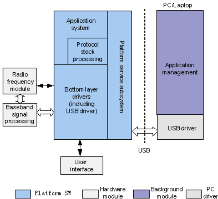
Figure 4-1 System architecture
