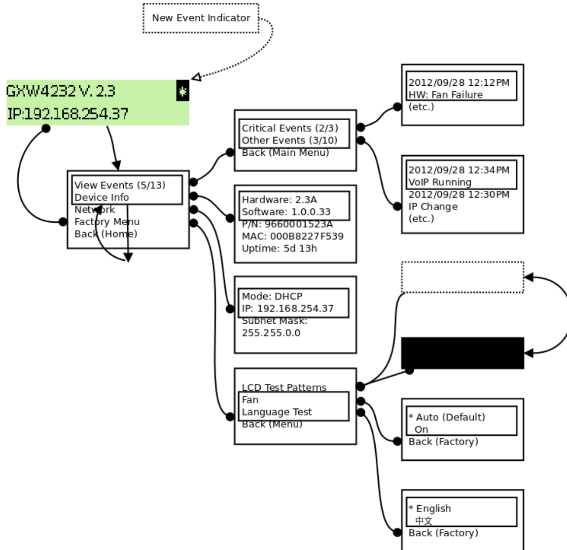
Figure 3: LCD Menu
