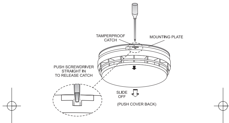
Figure 7: Removing the smoke alarm from the mounting plate
