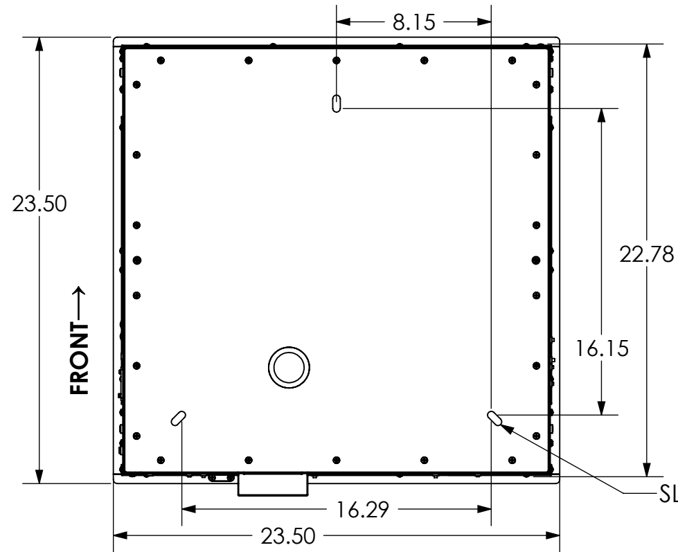
TOP VIEW
