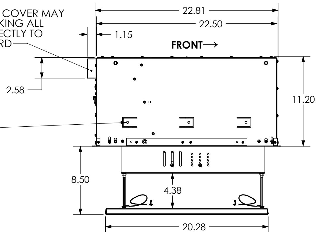
SIDE VIEW
