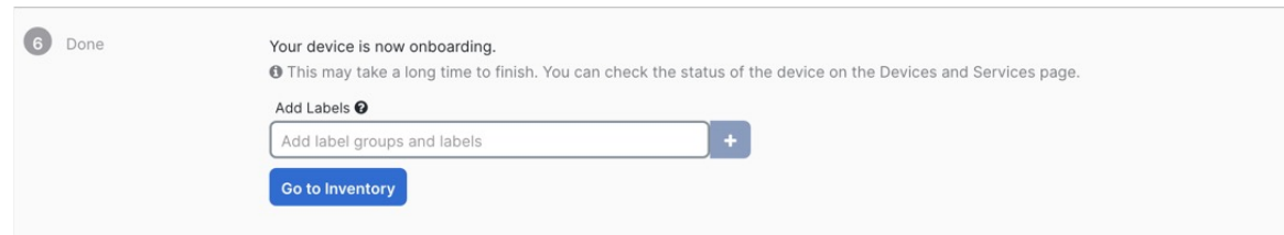
Figure 41: Done
