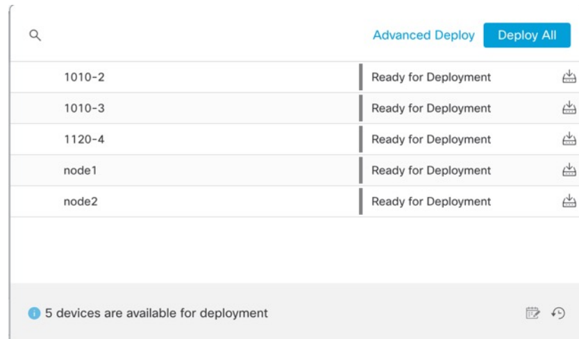
Figure 104: Advanced Deploy
