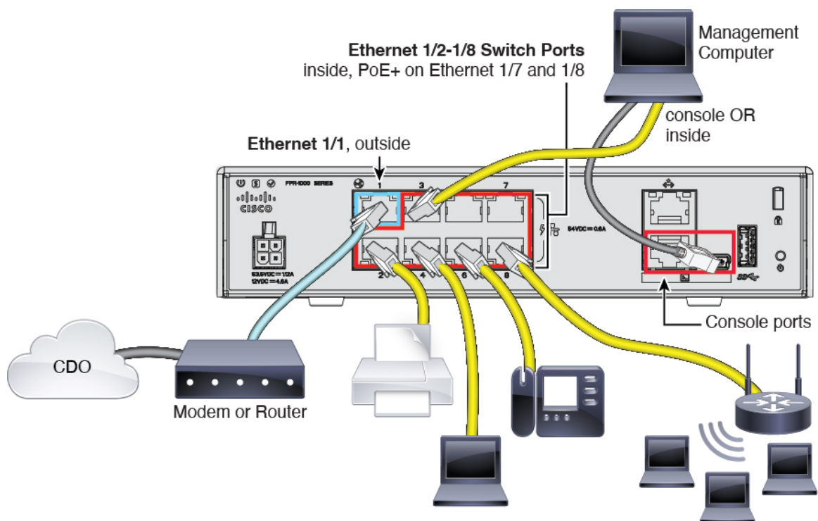
Figure 82: Cabling the Firepower 1010
