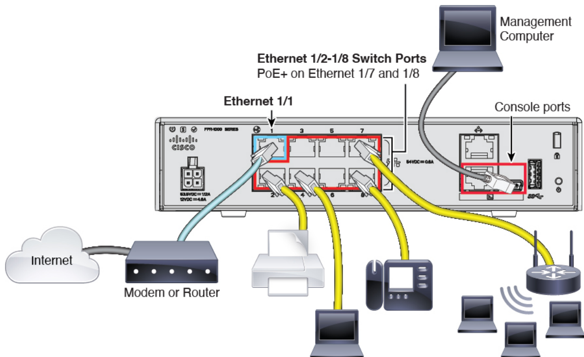
Figure 29: Cabling a Remote Management Deployment
