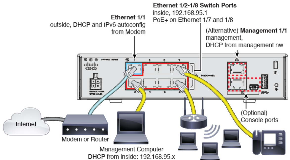
Figure 58: Cabling the Firepower 1010
