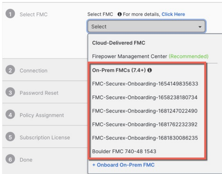
Figure 34: Select FMC
