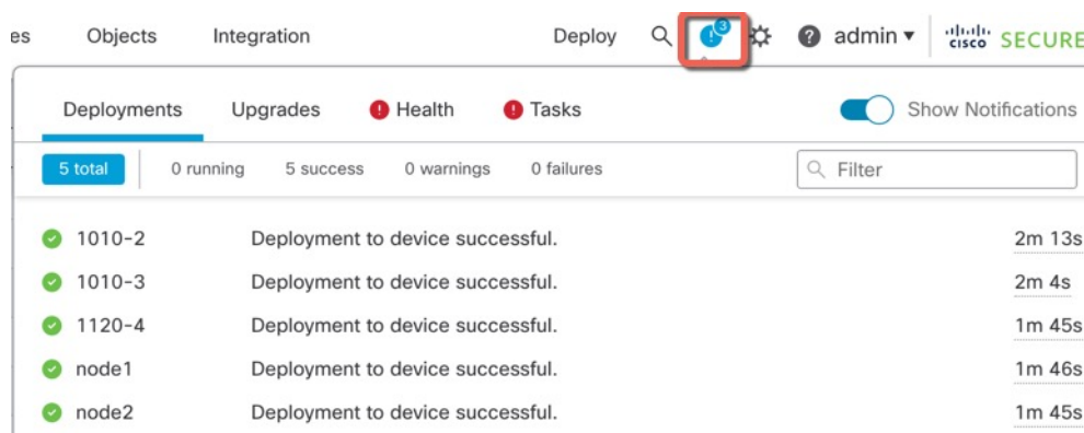
Figure 56: Deployment Status
