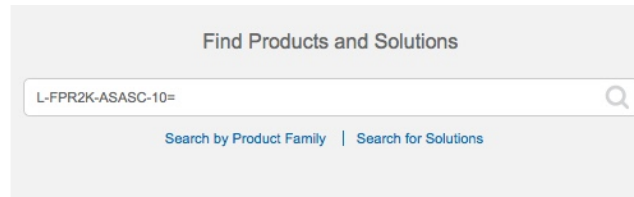
Figure 30: License Search
