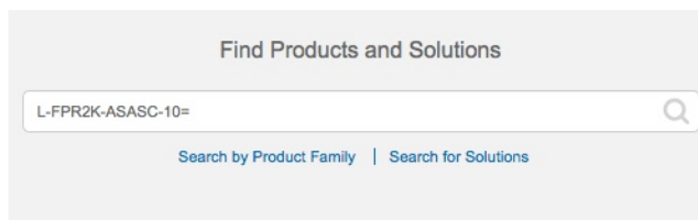
Figure 106: License Search
