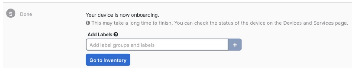
Figure 89: Done
