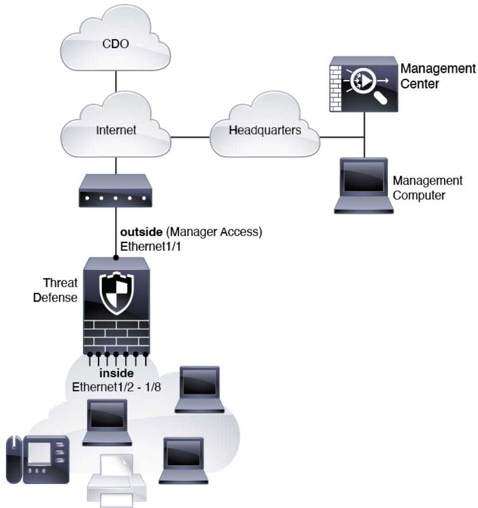
Figure 23: Low-Touch Provisioning Network
